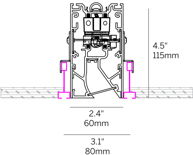
Recessed Trim for Slot Grid (RGTS)
