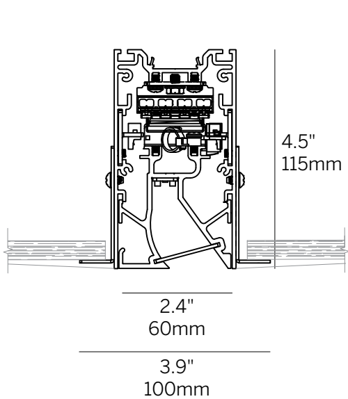
Recessed Plaster Trim (RPT)
