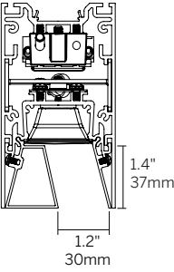
Recessed Elliptical Optic + Wall Graze (REO + WG)
