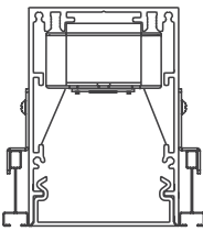
60LDL-RGTS Recessed Slot Grid 1•5
