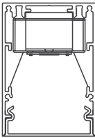
60LDL-SM Surface Mount 1•5
