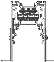
Recessed Plaster Trim
