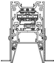
60PTL-RPT Recessed Plaster Trim 3•4•6•9•10
