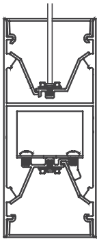
60LDI-S Suspended Direct / Indirect 1•2•5
