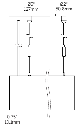
Power Feed + Suspension
