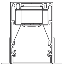
60LDL-RPT Recessed Plaster Trim 1•5
