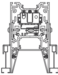
60PTL-RGTS Recessed Slot Grid 3•4•6•9•10
