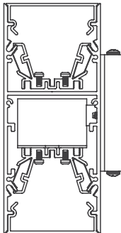
60LD/LDI-SW/SWM Mullion Mount Direct / Indirect 1•2•5
