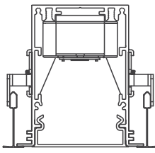
60LDL-RGT Recessed Grid Trim 1•5
