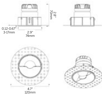
Plaster Trim (RPT)
