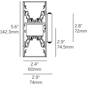
Surface Wall Mount (60LDI-SW)
