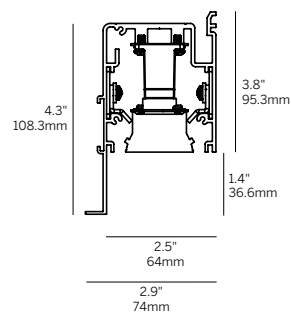
Wet Location (-WL) Regressed Opal Lens (ROL)
