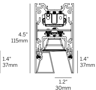
Recessed Elliptical Optic + Wall Graze (REO + WG)
