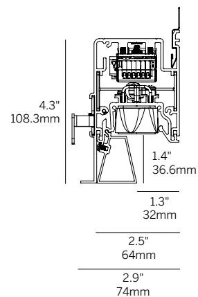
Recessed Elliptical Optic (REO + WG)
