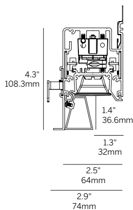
Recessed Louver (LW, RLB + WG)
