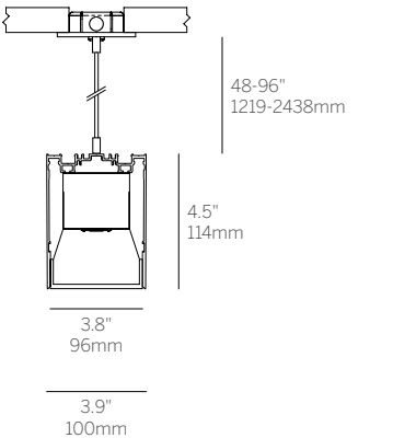
Suspended (100LDL)
