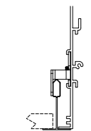
15/16" grid (RGT15)
