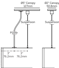
Power Feed + Suspension
