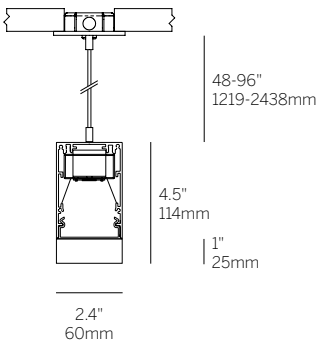
Suspended / Drop Diffuser (60LDL...DD)
