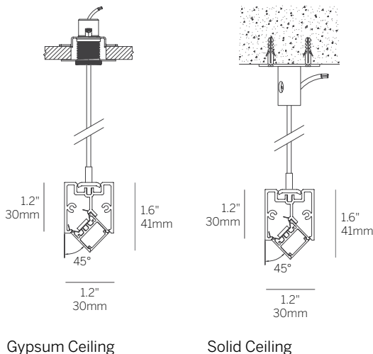
Power Feed
