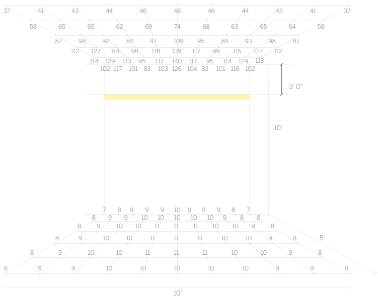
WG-20LWW-SRxT-...-S-...-H-935-MPL-W 10'-0" ceiling height
