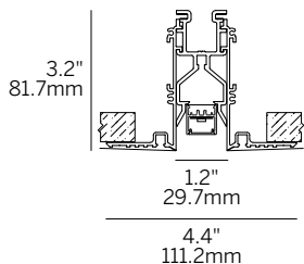
Recessed Plaster Trim (RPT)
