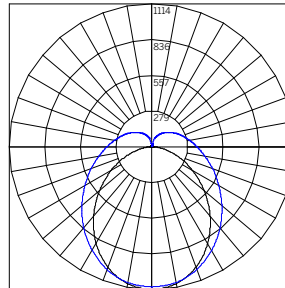
ILLUMINANCE - 48" ROD H 3500K WG-20LD-...-S-48-H-935-...-BDO-X-XXX-X-XX-W 1
