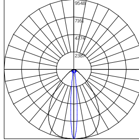
ILLUMINANCE - 48" NL16 H 3500K WG-20LD-...-S-48-H-935-...-NL16-X-XXX-X-XX-W 1
