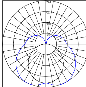
ILLUMINANCE - 48" BDO H 3500K WG-20LD-...-S-48-H-935-...-BDO-X-XXX-X-XX-W 1
