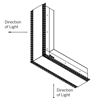
Plane To Plane Outside Corner (PPO)
