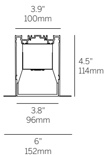
Recessed Plaster Trim (100LDL-RPT)
