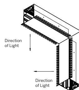
Plane To Plane Inside Corner (PPI)
