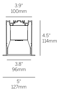
Recessed Bezel Trim / Grid Trim (100LDL-RBT/RGT)
