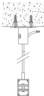
Solid Ceiling
