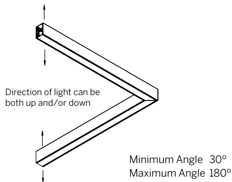
Pattern Corner
