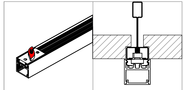
9/16" Bolt Slot (BS9T)
