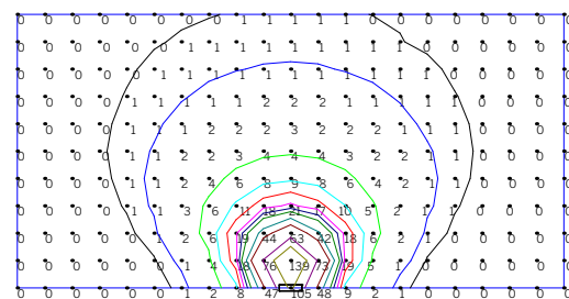
ISOILLUMINANCE DIAGRAM - 17W 3000K Asymmetric 1 EN66-RRWH-ME-106-17-CV-30-AS 2
