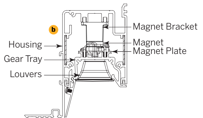
Cross Section of Gear Tray Seated in Housing
