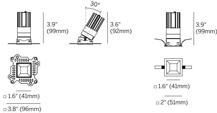
Plaster Trim (RPT) Cutout: 2" (50mm) Bezel Trim (RBT) Cutout: 1.8" (46mm)
