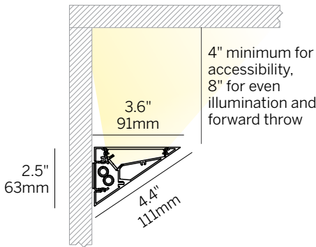
Wall Mounted Uplight (WCWL)
