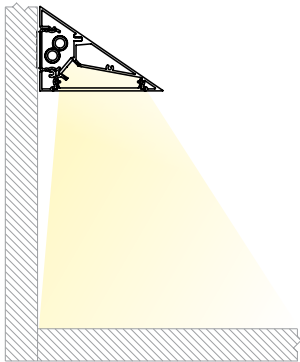
Wall Mounted Down Light (WCWLD)
