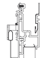
20 Linear Perimeter Flush Lens Grid Trim
