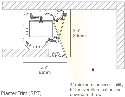
Plaster Trim (RPT)
