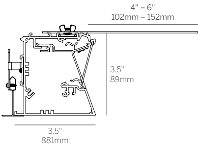
Grid Trim (RGT)
