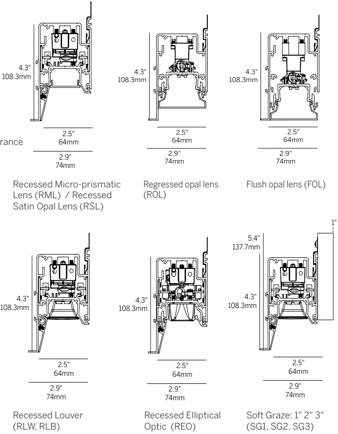
Recessed Louver
