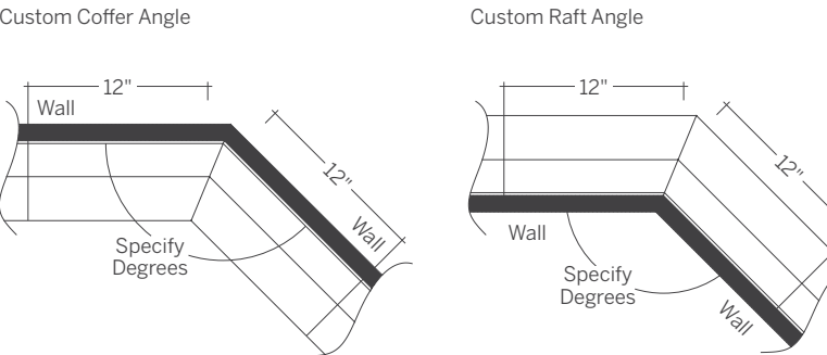
Custom Corners - Plan View
