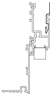
20 Linear Perimeter Regressed Lens Plaster Trim
