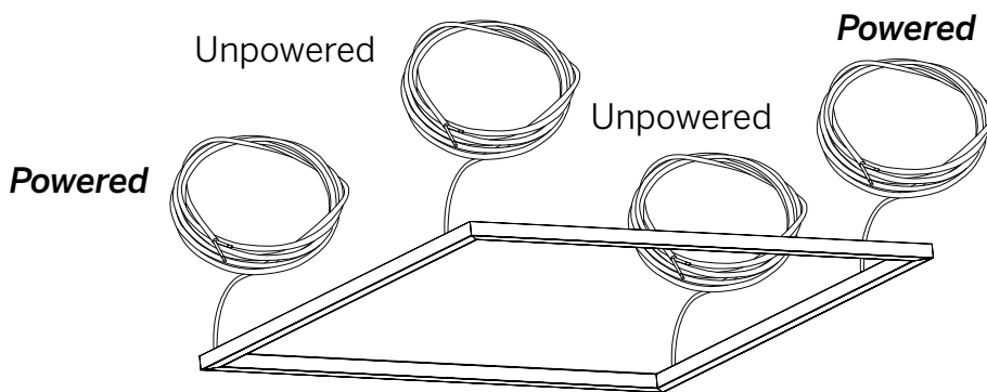
Dual Circuit Fixture Direct and Indirect lighting powered off of (2) Drivers. Direct and Indirect lighting may be operated and controlled separately.
