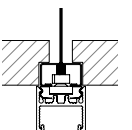
9/16" Bolt Slot Tegular clip (BS9T)
