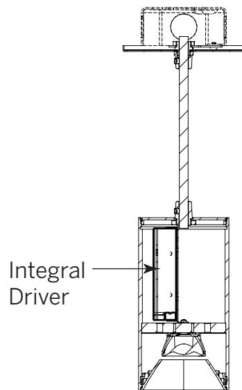
Cross-Section of Fixture
