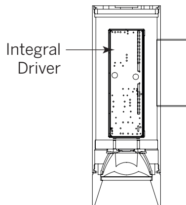
Cross-Section of Fixture
