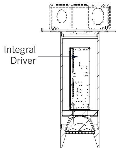
Cross-Section of Fixture
