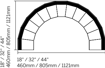
180° Corner Rafts (Outside) CR180 / 1832 - 3256 - 4478
