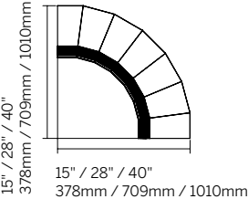
90° Corner Coffers (Inside) CC90 / 15 - 28 - 40
