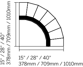
90° Corner Coffin (Inside) CC90 / 15 - 28 - 40
