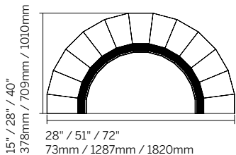
180° Corner Coffin (Inside) CC180 / 1528 - 2851 - 4072
