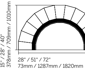
180° Corner Coffers (Inside) CC180 / 1528 - 2851 - 4072
