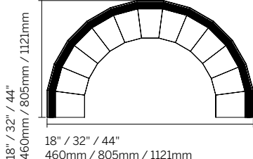
180° Corner Raft (Outside) CR180 / 1832 - 3256 - 4478
