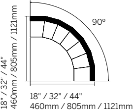
90° Corner Rafts (Outside) CR90 / 18 - 32 - 44
