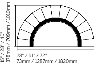
180° Corner Coffin (Inside) CC180 / 1528 - 2851 - 4072
