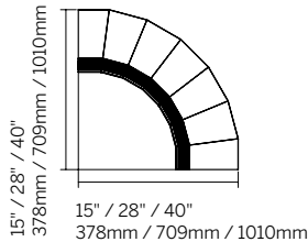
90° Corner Coffin (Inside) CC90 / 15 - 28 - 40
