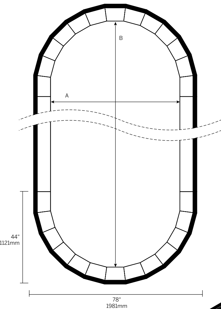
Bottom View
