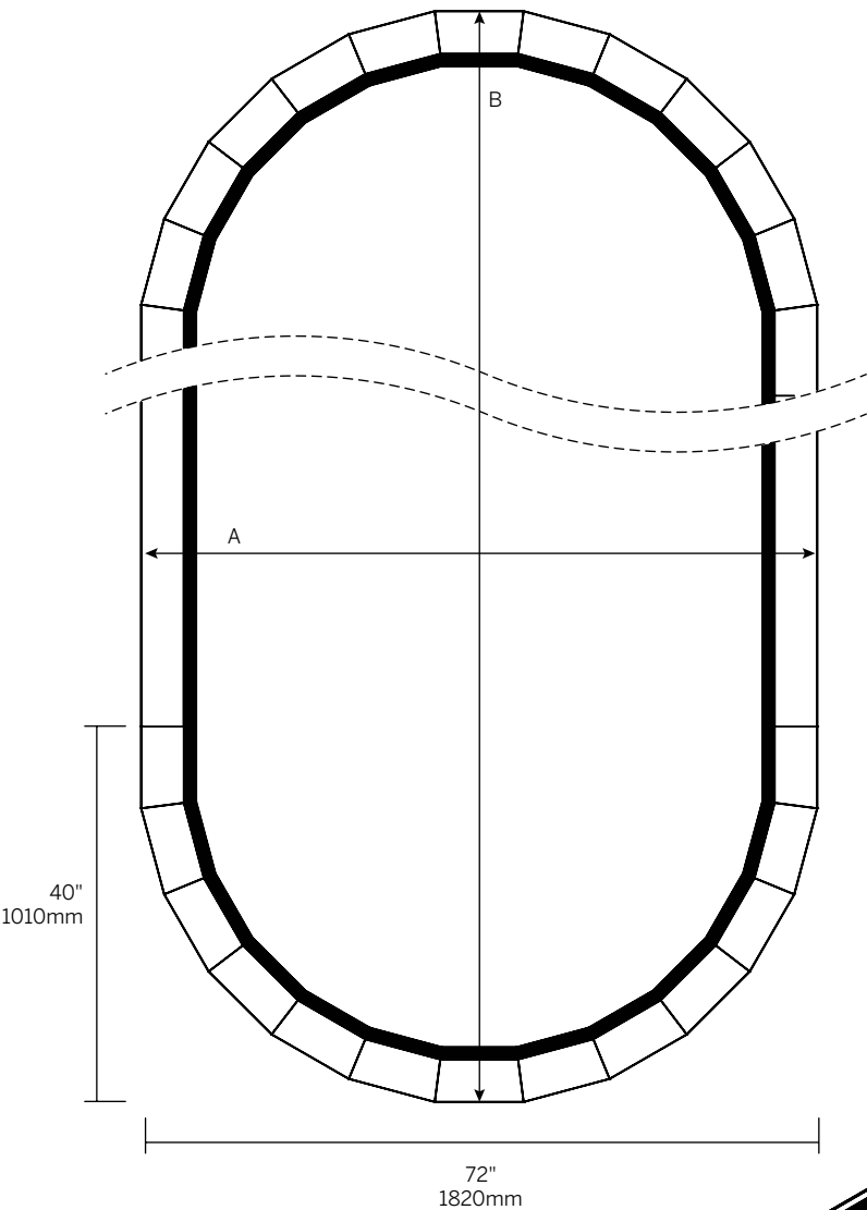
Bottom View
