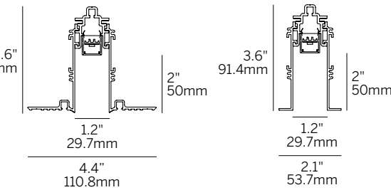
Recessed Plaster Trim (RPT)
