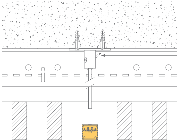
Detail @ 1:2
