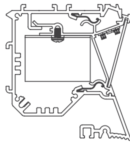
Z Cove Plaster Trim
