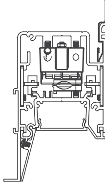
ProTools 60 Linear Perimeter Recessed
