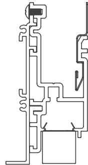
20 Linear Perimeter Flush Lens Bezel Trim
