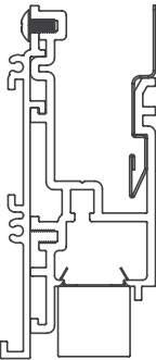
20 Linear Perimeter Flush Lens Return Trim
