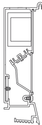
V Cove Plaster Trim
