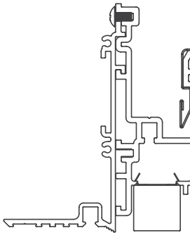
20 Linear Perimeter Flush Lens Plaster Trim
