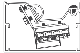
Box Cove 2 Surface/Mullion Mount
