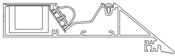
Edgeless Cove Plaster Trim
