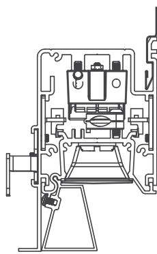
ProTools 60 Linear Wall Graze Recessed
