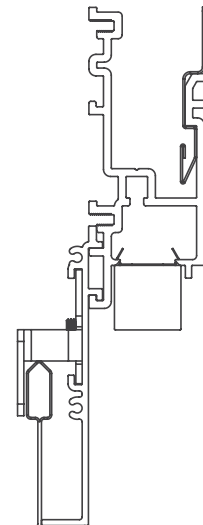
20 Linear Perimeter Regressed Lens Grid Trim
