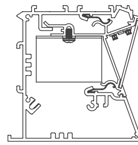
Z Cove Grid Trim
