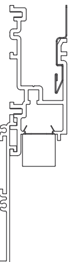
20 Linear Perimeter Regressed Lens Return Trim
