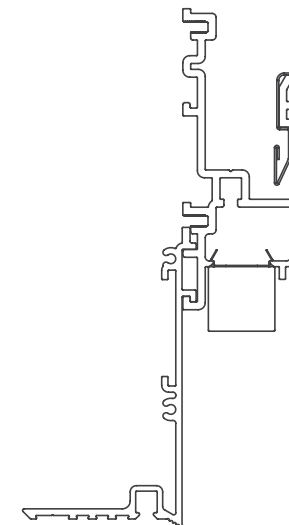
20 Linear Perimeter Regressed Lens Plaster Trim
