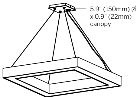
Center canopy with remote driver
