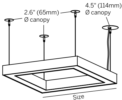
Straight cables with remote driver
