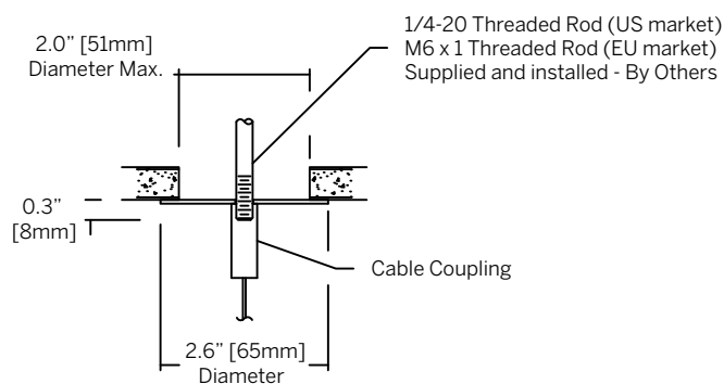
Mounting Option - Non Power Threaded Rod installed to structural ceiling (By Others)
