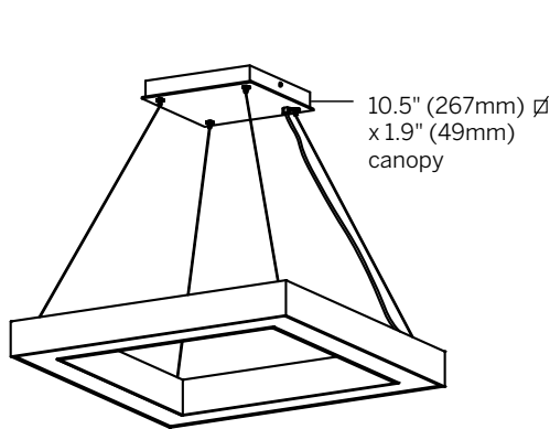
Center canopy with integral driver
