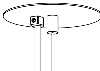
Mounting Option Power Octagon Box (By Others) Installed in drywall, wood or concrete ceiling
