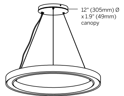
Center canopy with integral driver
