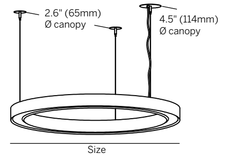
Straight cables with remote driver
