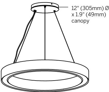
Center canopy with integral driver
