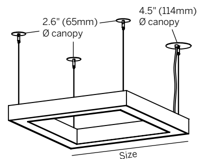
Straight cables with remote driver
