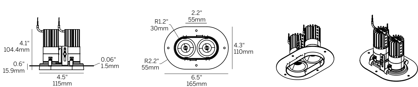
Oval Twin Trim with Wood Ceiling Trim (OTTWC)
