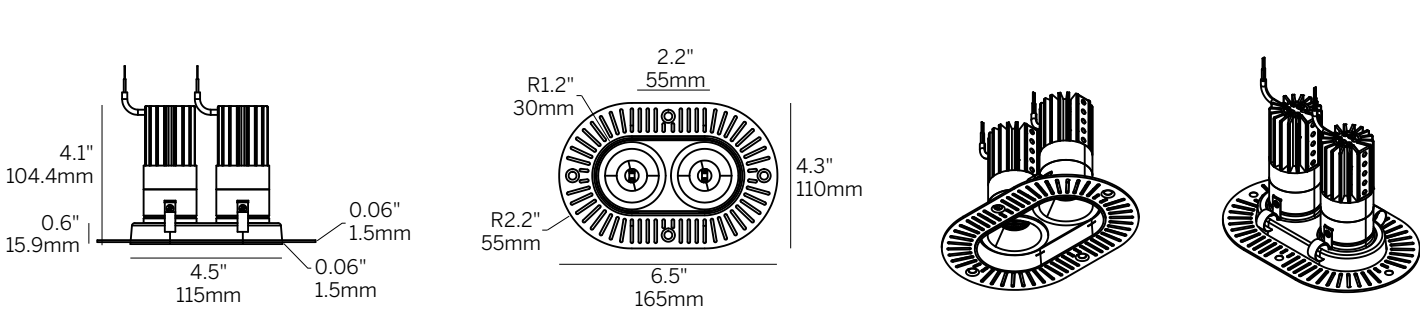
Oval Twin Trim with Plaster Trim (OTTPT)
