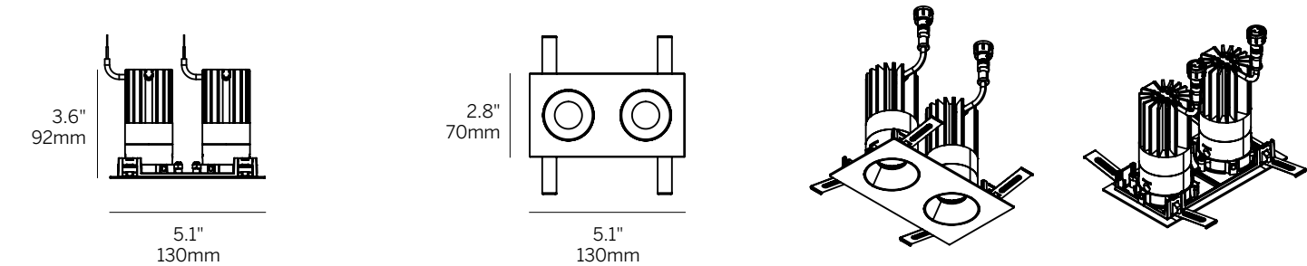
Rectangular Twin Trim with Bezel Trim (RTTBT)
