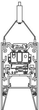
60PTLWW Recessed Wall Wash 9
