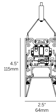
Recessed Micro-prismatic Lens (RML)
