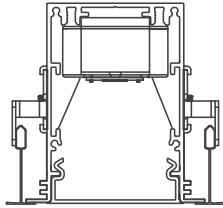
60LDL-RGT Recessed Grid Trim 1•4
