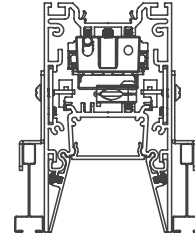
60PTL-RGTS Recessed Slot Grid 3·5·7·8
