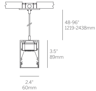
Suspended / Drop Diffuser (60LDL...DD)
