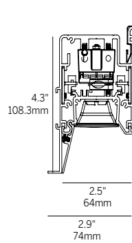
Recessed Louver (RLW, RLB)
