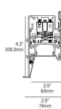
Recessed Micro-prismatic Lens (RML)
