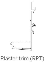
Plaster trim (RPT)
