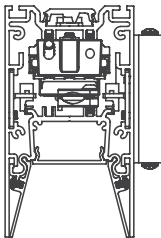
60PTLDI-SW/SWM Wall / Mullion Mount Direct/Indirect 3•5•6•7
