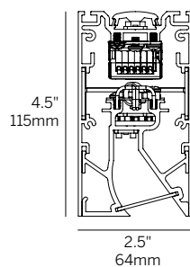
Recessed Lens + Wall Wash (LML + WW)
