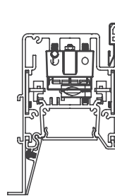
60PTLP Recessed Perimeter 3•6•7
