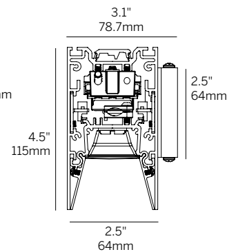
Recessed Louver (RLW, RLB)
