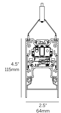
Regressed Opal Lens (ROL)
