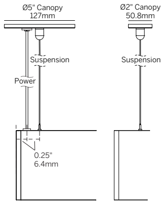
Power Feed + Suspension
