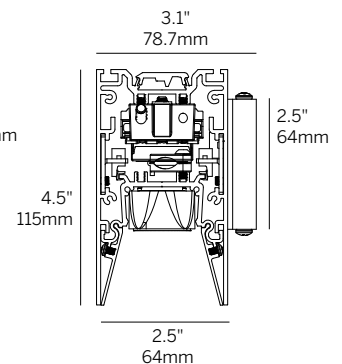
Recessed Elliptical Optic (REO)
