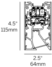
Recessed Lens + Wall Wash (LML + WW)
