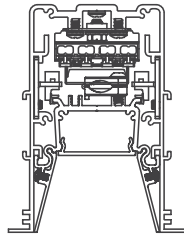
60PTL-RBT Recessed Bezel Trim 3•5•7•8
