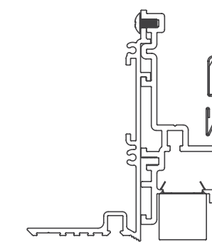
20 Linear Perimeter Flush Lens Plaster Trim
