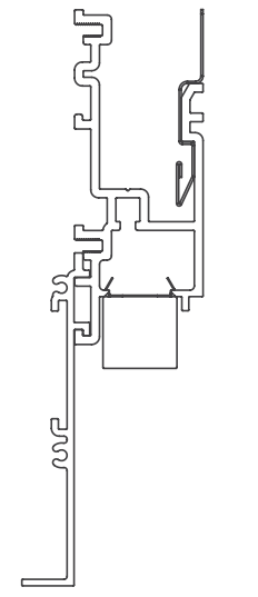
20 Linear Perimeter Regressed Lens Bezel Trim
