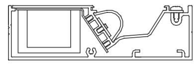
Box Cove Surface Mount
