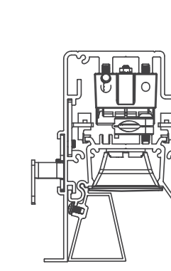
ProTools 60 Linear Wall Graze Recessed
