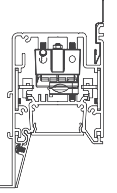
ProTools 60 Linear Perimeter Recessed
