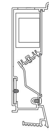
V Cove Plaster Trim
