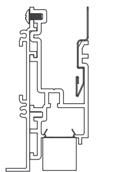
20 Linear Perimeter Flush Lens Bezel Trim
