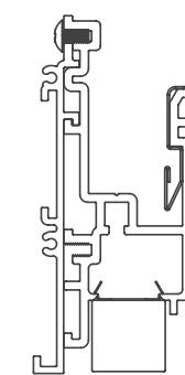
20 Linear Perimeter Flush Lens Return Trim
