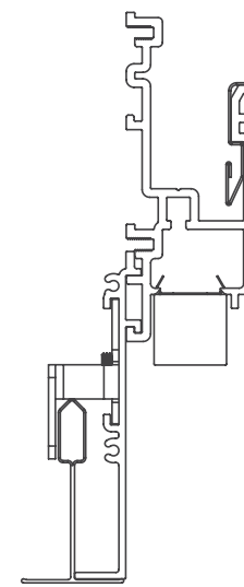
20 Linear Perimeter Regressed Lens Grid Trim
