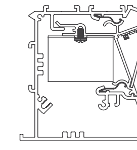
Z Cove Grid Trim
