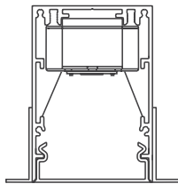
60LDL-RPT Recessed Plaster Trim 1-4
