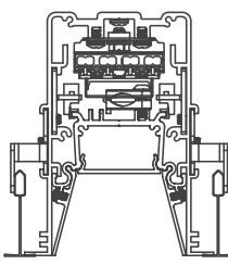
60PTL-RGT Recessed Grid Trim 3-5-7-8
