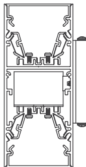
60LD/LDI-SW/SWM Mullion Mount Direct / Indirect 1-2
