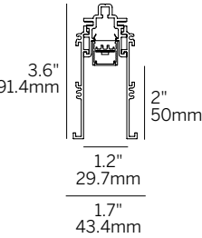
Recessed Return Trim (RRT)
