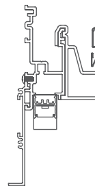
20LPRSG-RBT Regressed Bezel Trim Soft-graze 1•2•3•4•5
