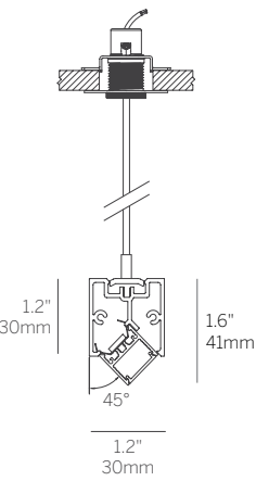
Gypsum Ceiling
