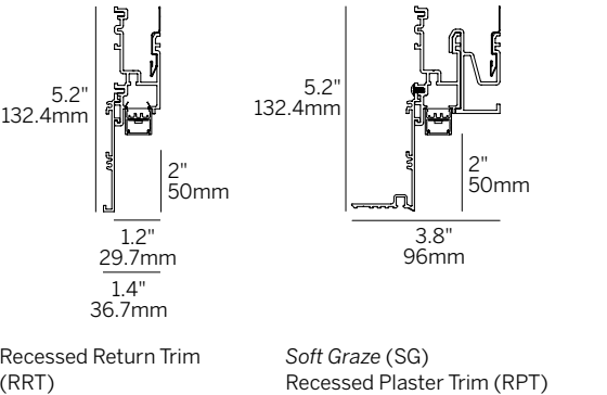
Recessed Plaster Trim (RPT)
