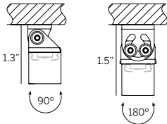
Adjustable Brackets (A90 / A180)
