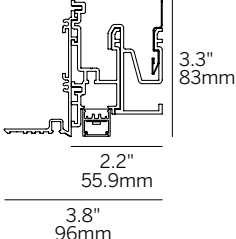
Soft Graze (SG) Recessed Plaster Trim (RPT)
