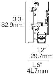
Recessed Bezel Trim (RBT) Recessed Grid Trim (RGT9/RGT15)
