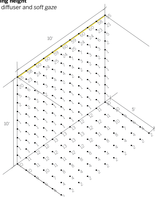
WG-20LPRSG-...-S-...-P3-935-OD-W 20'-0" ceiling height Satin opal diffuser and soft gaze
