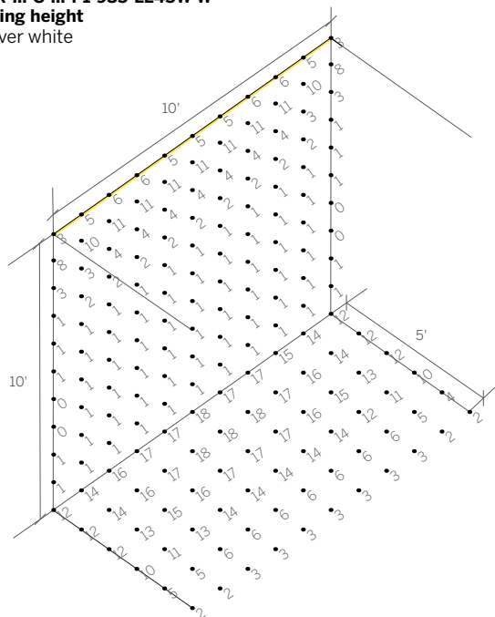
WG-20LPR-...-S-...-P3-935-LL45W-W 20'-0" ceiling height Linear louver white
