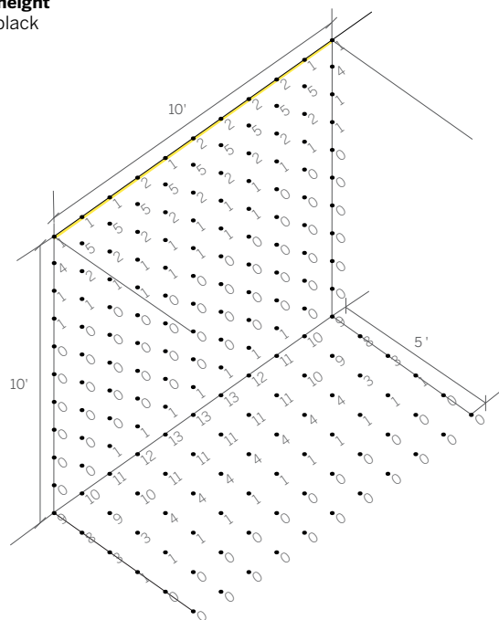
WG-20LPR-...-S-...-P3-935-LL45B-W 20'-0" ceiling height Linear louver black
