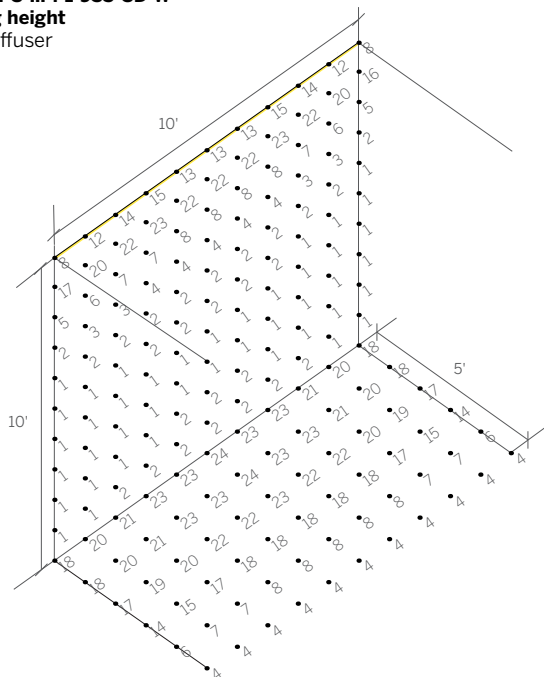
WG-20LPR-...-S-...-P3-935-SD-W 20'-0" ceiling height Satin clear diffuser
