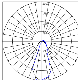
ILLUMINANCE - 48" LL45W P3 3500K WG-20LPR-...-S-48-P3-935-...-LL45W-W 1
