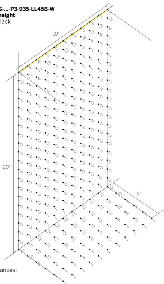
WG-20LPRSG-...-S-...-P3-935-LL45B-W 20'-0" ceiling height Linear louver black and soft gaze
