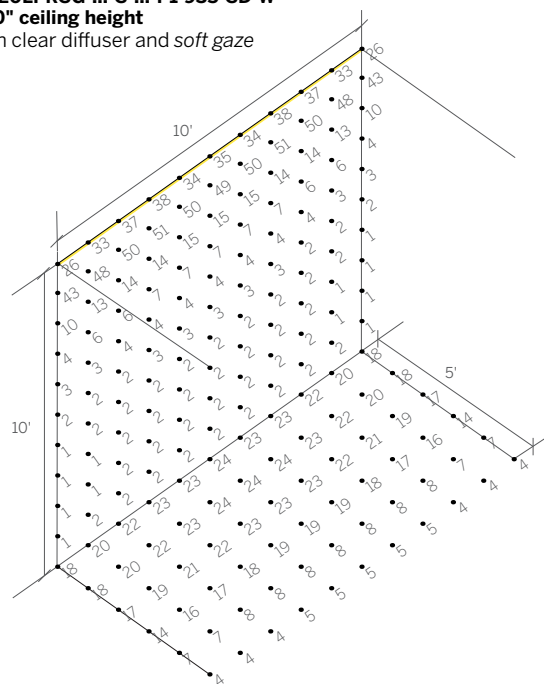
WG-20LPRSG-...-S-...-P3-935-SD-W 20'-0" ceiling height Satin clear diffuser and soft gaze
