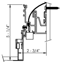
Recessed Grid Trim Soft-Graze
