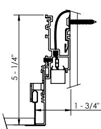
Recessed Grid Trim
