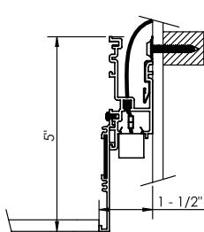
Recessed Return Trim
