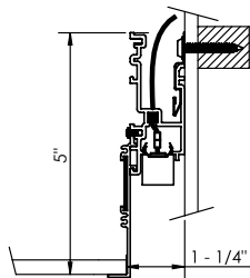
Recessed Bezel Trim
