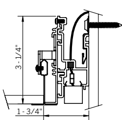
Recessed Grid Trim
