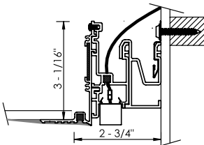
Recessed Plaster Trim Soft-Graze
