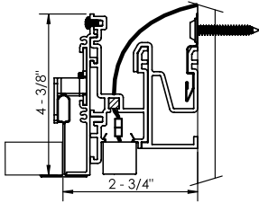
Recessed Grid Trim Soft-Graze
