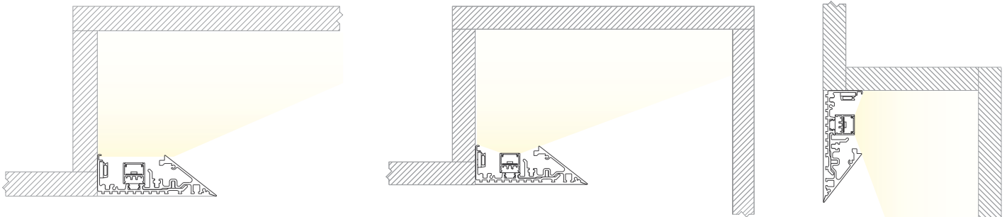
Gypsum Ceiling Mounting Options 4" minimum offset, 12" typical offset
