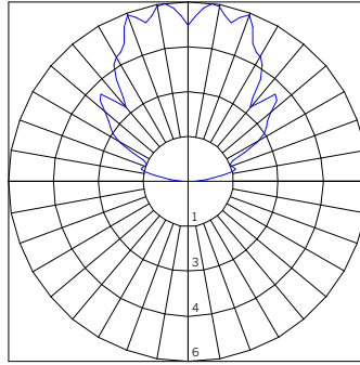
Beam Angle (0-180) = 113.2 Beam Angle (90-270) = 113.2
