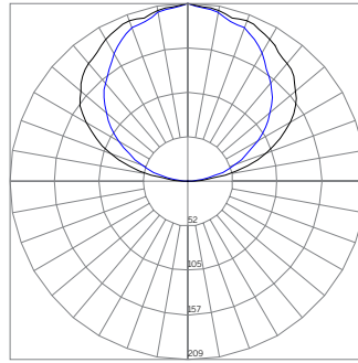
Beam Angle (0-180) = 114.2 Beam Angle (90-270) = 137
