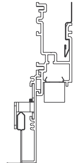
20 Linear Perimeter Regressed Lens Grid Trim
