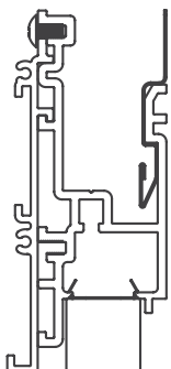
20 Linear Perimeter Flush Lens Return Trim
