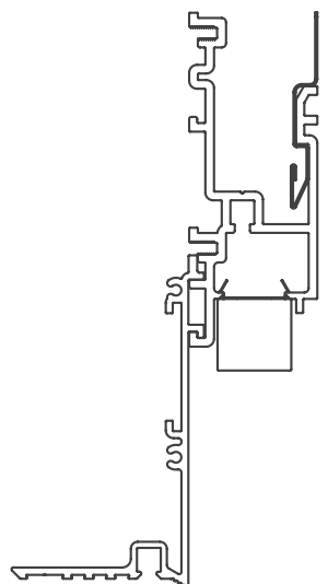
20 Linear Perimeter Regressed Lens Plaster Trim
