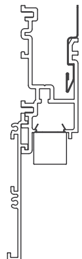
20 Linear Perimeter Regressed Lens Return Trim
