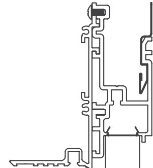
20 Linear Perimeter Flush Lens Plaster Trim
