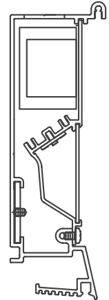
V Cove Plaster Trim
