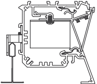
Z Cove Grid Trim
