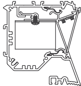
Z Cove Plaster Trim
