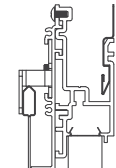
20 Linear Perimeter Flush Lens Grid Trim
