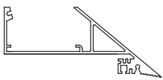
Edgeless Nose Cove Plaster Trim
