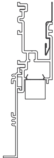
20 Linear Perimeter Regressed Lens Bezel Trim
