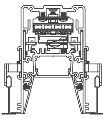
60PTL-RGT Recessed Grid Trim 4•6•8•9
