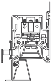
60PTLWG Recessed Wall Graze 7•8
