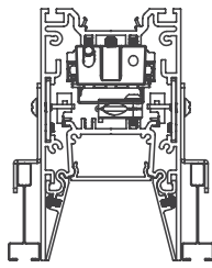
60PTL-RGTS Recessed Slot Grid 4•6•8•9
