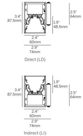
Surface Wall Mullion Mount (60LD/60LI-SWM)
