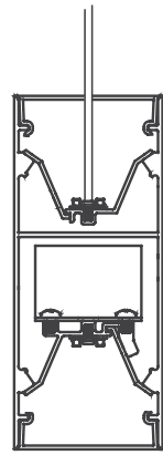
60LDI Suspended Direct / Indirect 1•2•3•5
