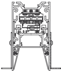
60PTL-RPT Recessed Plaster Trim 4•6•8•9
