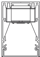
60LDL-SM Surface Mount 1•3•5
