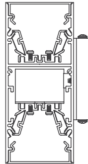
60LD/LDI-SW/SWM Mullion Mount Direct / Indirect 1•2•3
