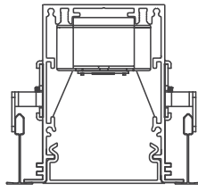
60LDL-RGT Recessed Grid Trim 1•3•5
