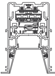
60PTL-RBT Recessed Bezel Trim 4•6•8•9
