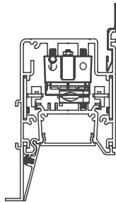
60PTLP Recessed Perimeter 4•7•8
