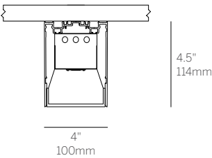
Surface (100LDL-SM)
