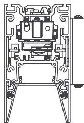
60PTLDI-SW/SWM Wall / Mullion Mount Direct/Indirect 4•6•7•8
