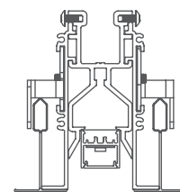
20LRF-RGT Flush Grid Trim 1·2·3·4·5·6
