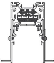
Recessed Plaster Trim (WG-60PTL-RPT)
