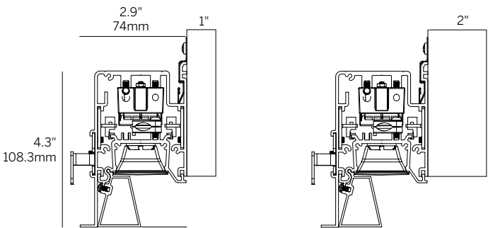
Recessed Louver (SG1 + RLW, RLB)
