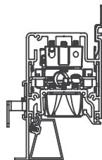
Recessed Lens + Wall Graze (REO + WG)
