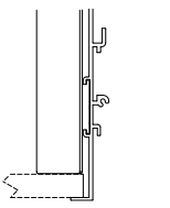
Recessed trim (RBT)
