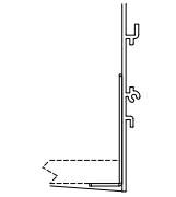
Plaster trim (RPT)
