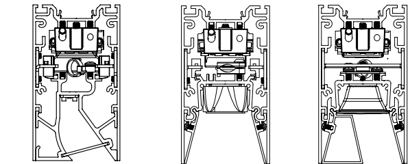
Recessed Lens + Wall Wash (LML + WW) Recessed Narrow Optic (RNO) Wall Graze (WG)
