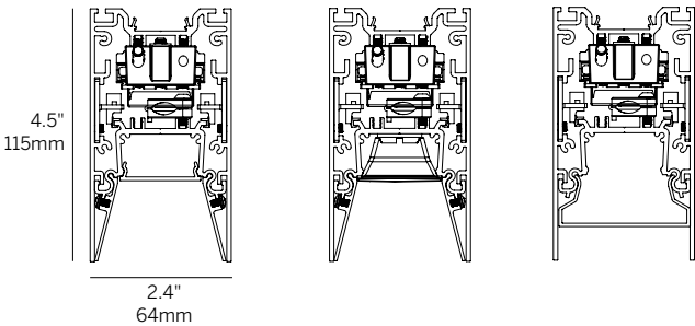
Recessed Micro-prismatic Lens (RML) Recessed Louver (RLW, RLB) Regressed Opal Lens (ROL)
