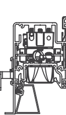
Recessed Lens + Wall Graze (REO + WG)
